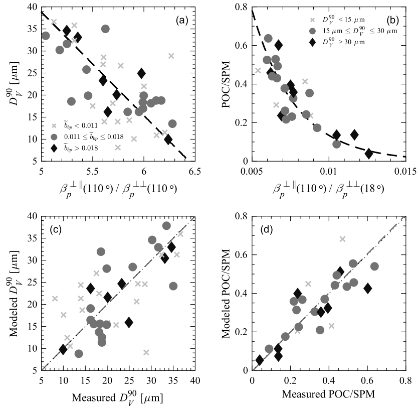
Fig. 12. (a) Particle size parameter D_v^{90} and (b) particle composition parameter POC/SPM as functions of polarized light scattering metrics for seawater samples. Linear regression (a) and exponential regression (b) functions are plotted with black dashed lines. Bottom panels (c), (d) present model performance using model-derived values from regression from the panel above and the measured D_v^{90} or POC/SPM , respectively. A type II linear regression of modeled versus measured data is plotted with a gray dashed line. A 1:1 dotted line is also plotted, which is nearly indistinguishable from the regression line. Data in (a), (c) are indicated by particulate composition-related parameter \tilde{b}_{bp} as shown in legend in (a), while (b), (d) are indicated by particle size parameter D_v^{90} as shown in legend in (b).
