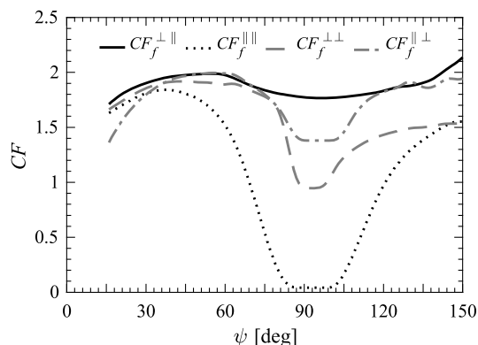
Fig. 2. Final correction functions CF_f^{ee}(\psi) for LISST-VSF measurements of each polarized light scattering measurement combination, as indicated in legend, over the angular range 16°–150° determined from analysis of 100, 200, and 400 nm polystyrene bead suspensions.
